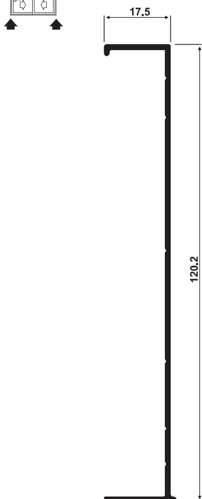
MARCO LATERAL
