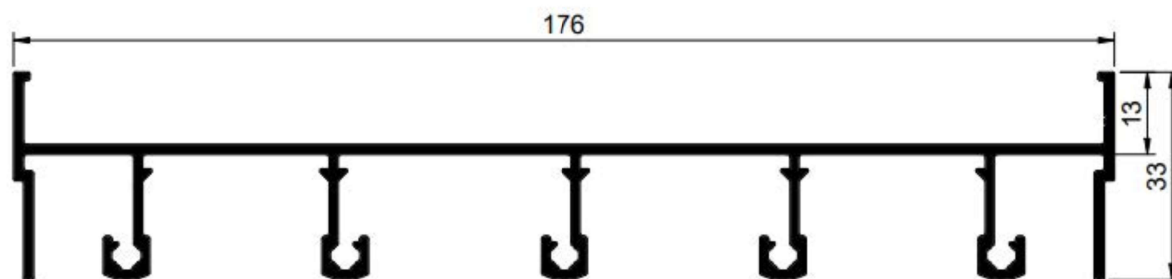
SU-605 1,749 kg/m
