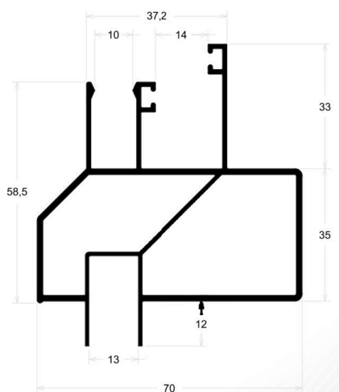
GR-48 1,357 kg/mt
