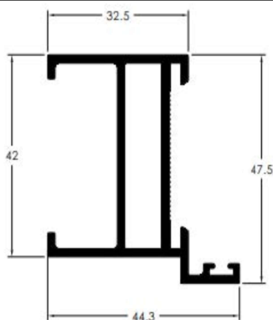
42-012 0,853kg/m
