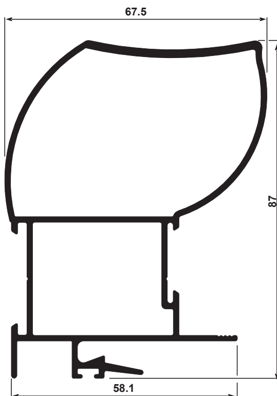
LG-137 1,526 kg/m
