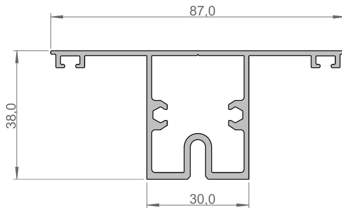
AT-204 - 1,038 kg/mt
