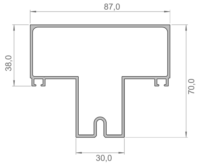
AT-400 - 1,433 kg/mt Coluna Central 70mm
