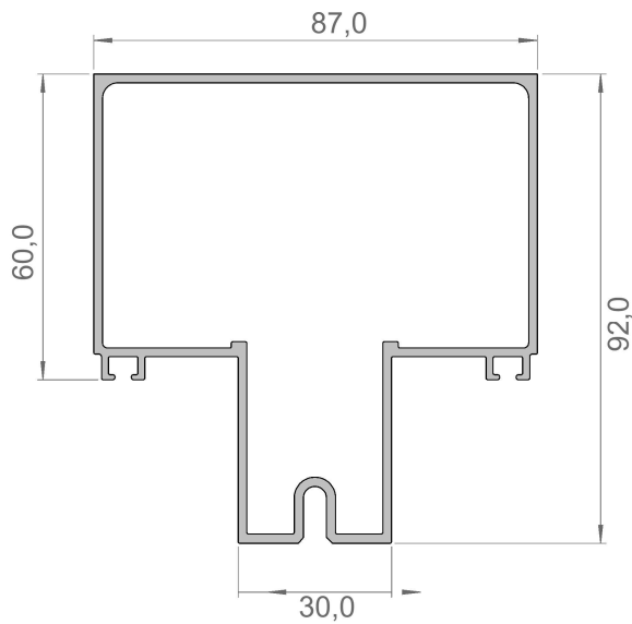
AT-200 - 1,824 kg/mt Coluna Central 92mm
