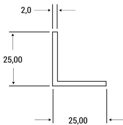
Cantoneira
