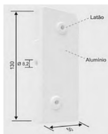
Dobradiça superior injetada
