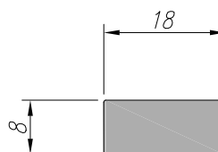
ES-1316 BARRA CHATA 0,390 kg/m
