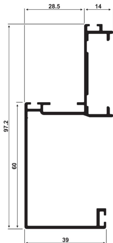
FC-243 FC-243 1,009 kg/m
