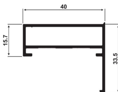
FC-261 FC-261 0,516 kg/m
