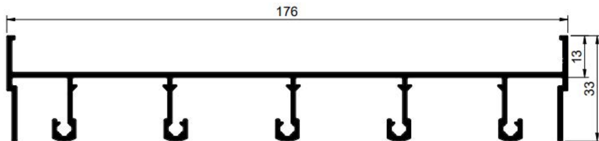
SU-605 1,749 kg/m
