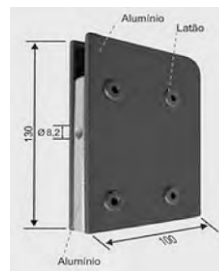
MAX Dobradiça superior
