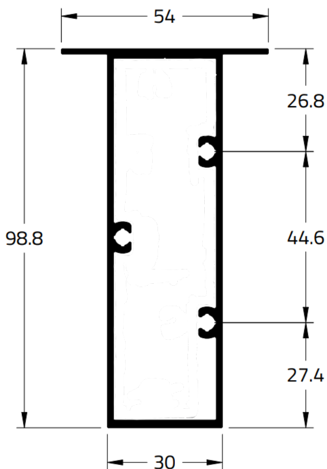
CHR-033 1,171 Kg/m
