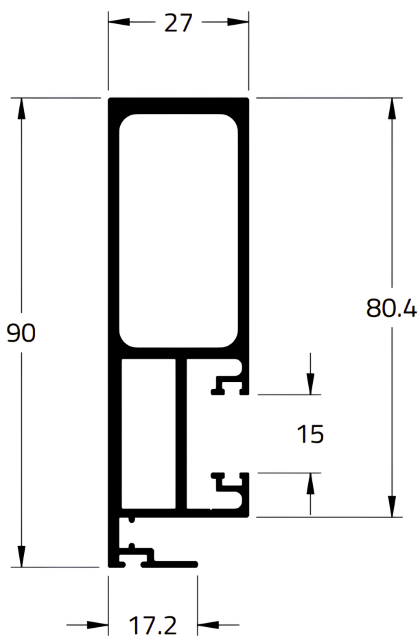
CHR-213 1,612 Kg/m
