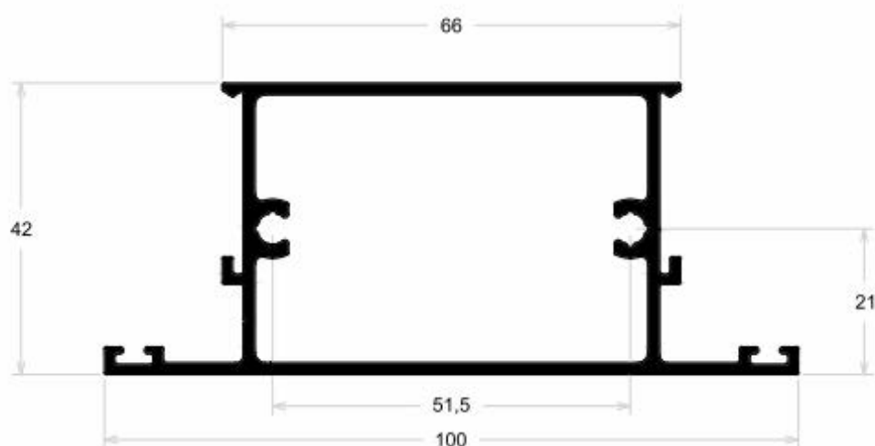
Travessa 100mm
