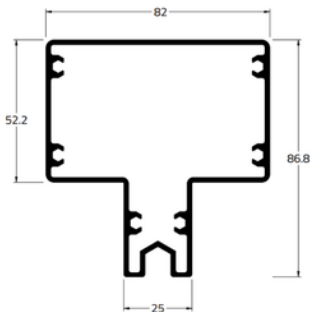
LUVA MONTANTE CENTRAL 295MM PS306 LUV327
