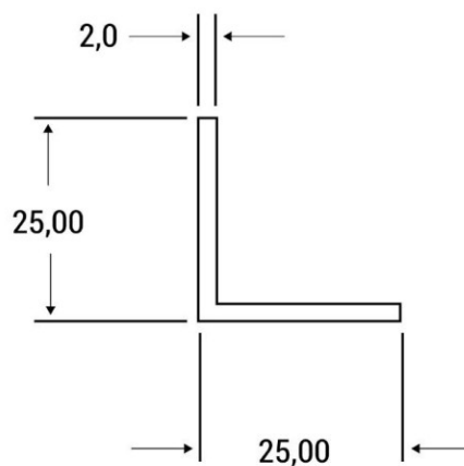
Cantoneira
