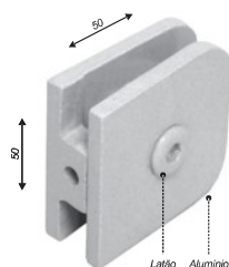
Suporte central 50x50mm
