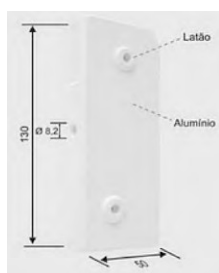
Dobradiça superior injetada
